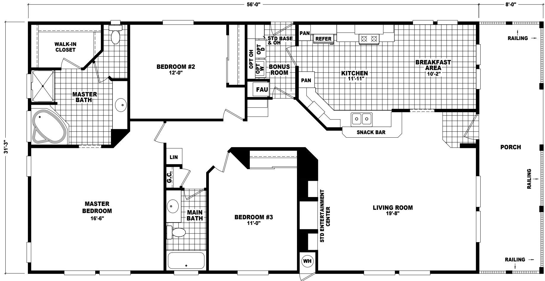
MODEL: FPS-3264A APPROXIMATELY 2000 SQ. FT.* 3 BEDROOM, 2 BATH *INCLUDES PORCH
